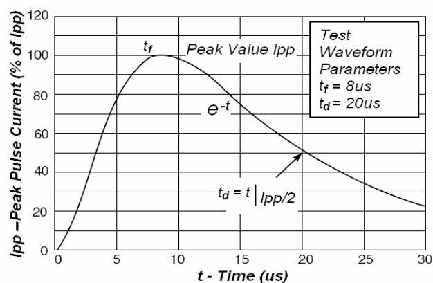
Fig1. Pulse Waveform
