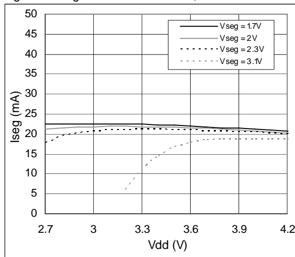
Figure 8. Segment Current vs. VDD; V_{Rset} = 2.8\text{V}
