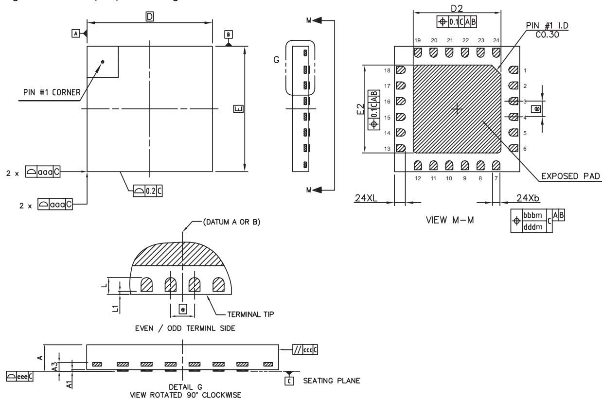
Figure 22. TQFN(4x4)-24 Package
