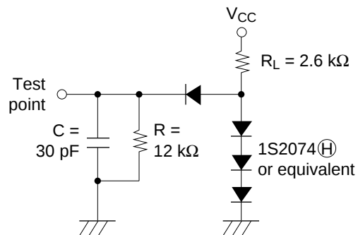
Figure 99 Timing Load Circuit
