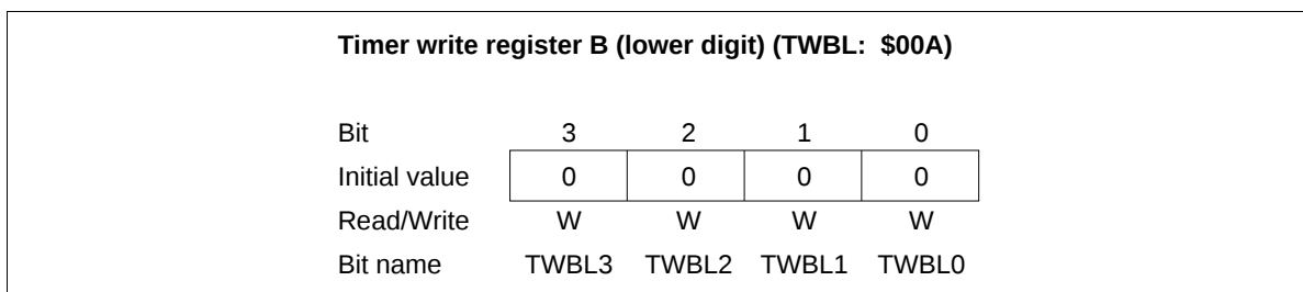
Figure 46 Timer Write Register B Lower Digit (TWBL)
