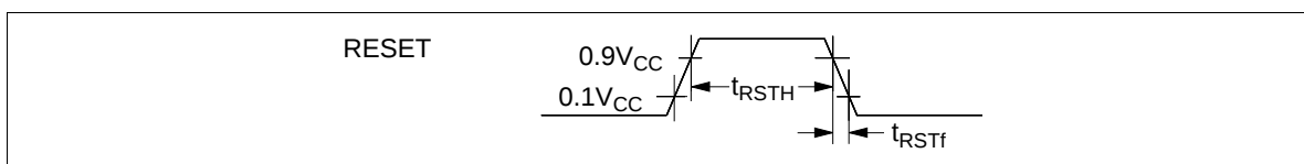
Figure 96 Reset Timing
