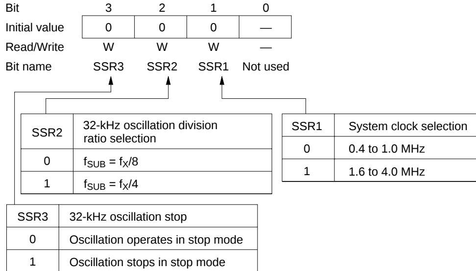
Figure 26 System Clock Select Register
