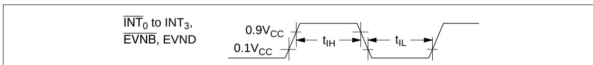
Figure 95 Interrupt Timing
