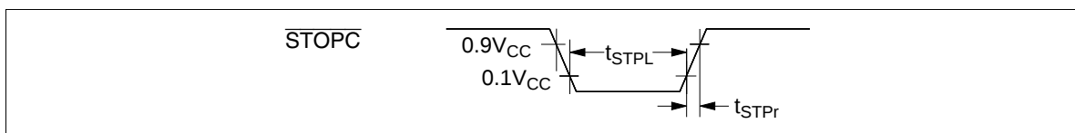
Figure 97 \overline{STOPC} Timing
