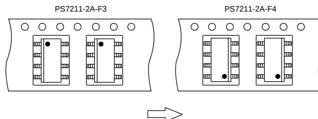
TAPE DIRECTION
