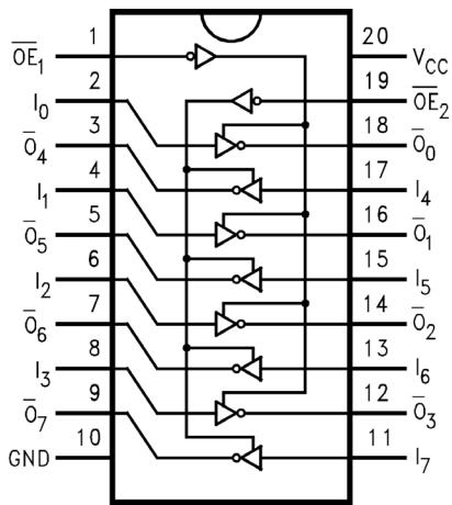
Figure 1. Connection Diagram
