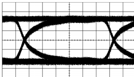
Output Waveform
