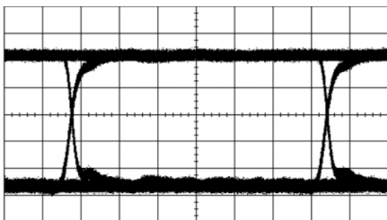
Input Waveform
