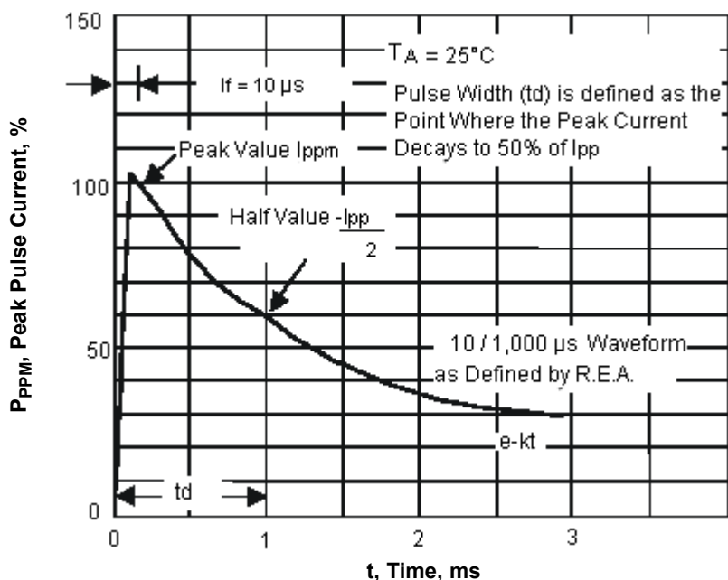
Fig. 3-Pulse Waveform
