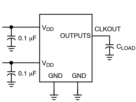
Figure 9. Test Circuit #1
