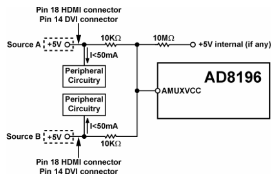
Figure 28. Suggested AMUXVCC Power Scheme
