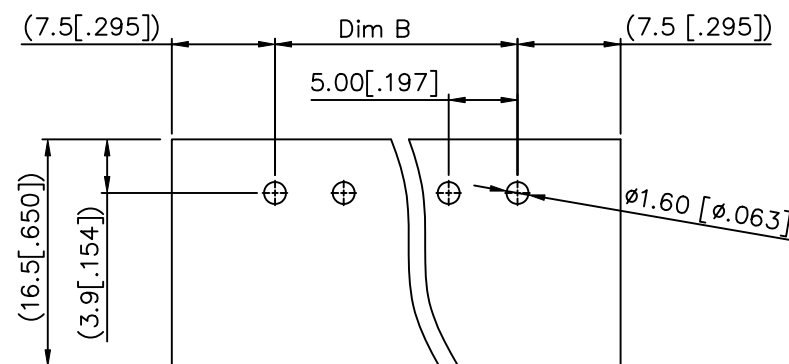
PCB LAYOUT
