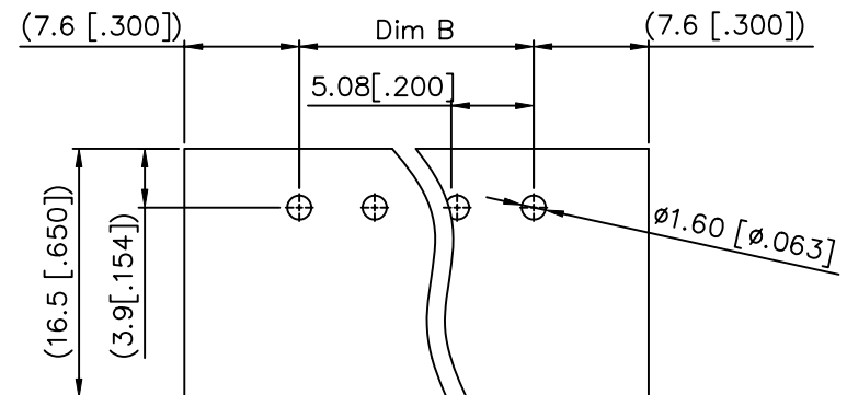
PCB LAYOUT
