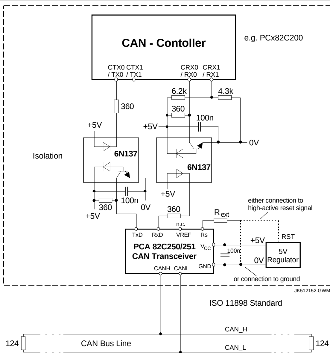
Programming of the Output Control Register (example) Output Control TX0 push-pull, dominant = low e.g. 1A hex Fig. 4 Application example for an interface with galvanic isolation using optocouplers
