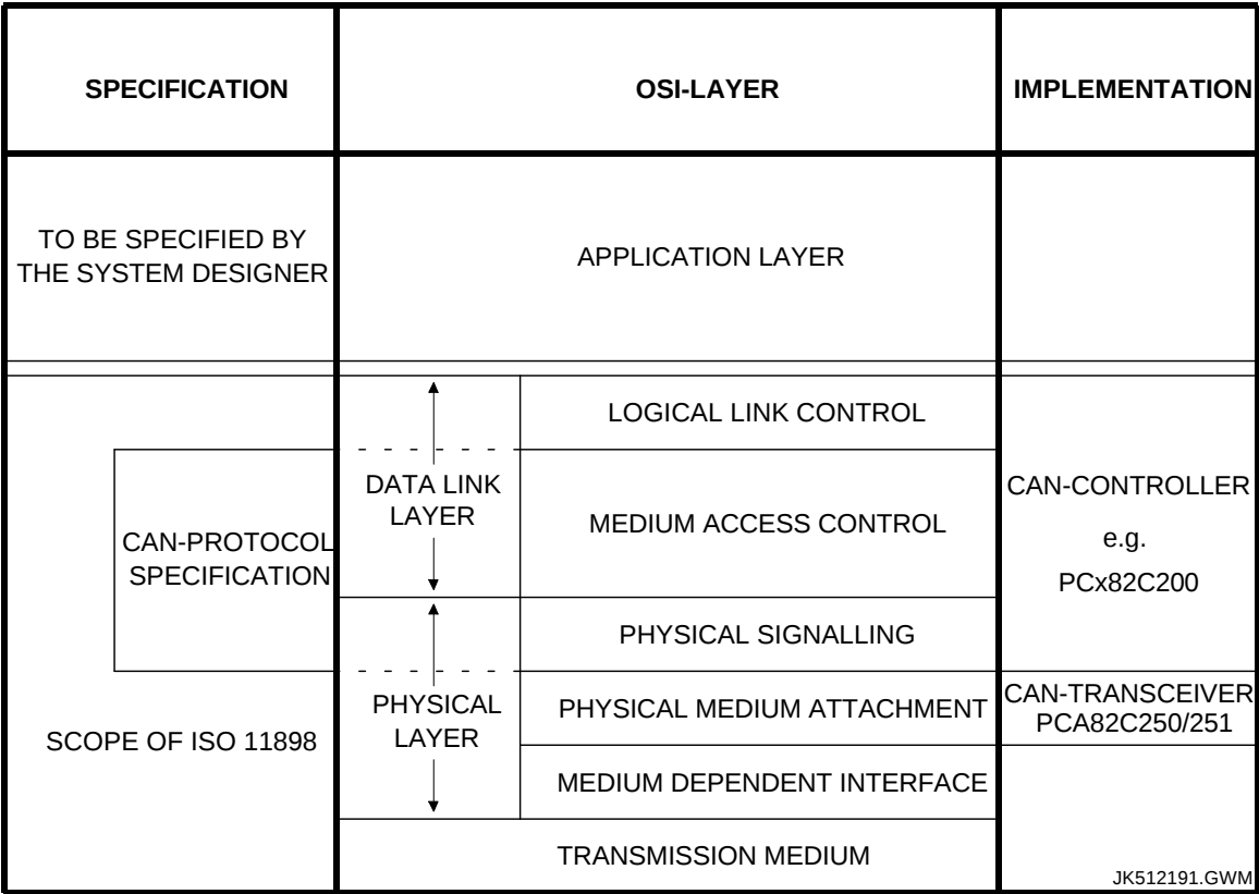
Fig. 1 Layered architecture of CAN
