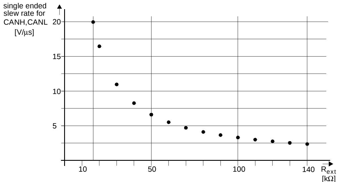
Fig. 5 Diagram: Slew rate versus slope control resistance value
