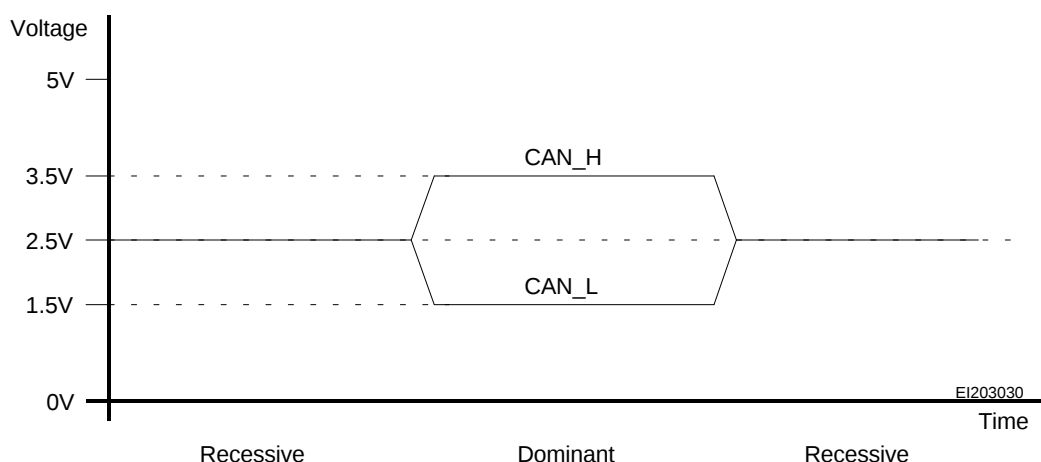
Fig. 2 Nominal bus levels according to ISO 11898
