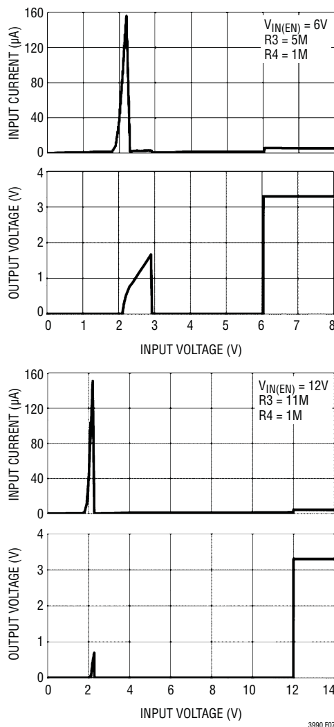
Figure 7. V_{IN} Start-Up of Front Page Application with V_{OUT} = 3.3V , No-Load Current, and V_{IN(EN)} programmed as in Figure 6.
