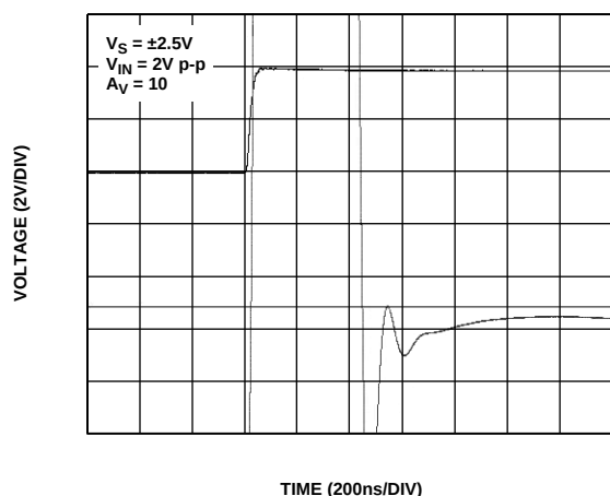
Figure 24. Settling Time
