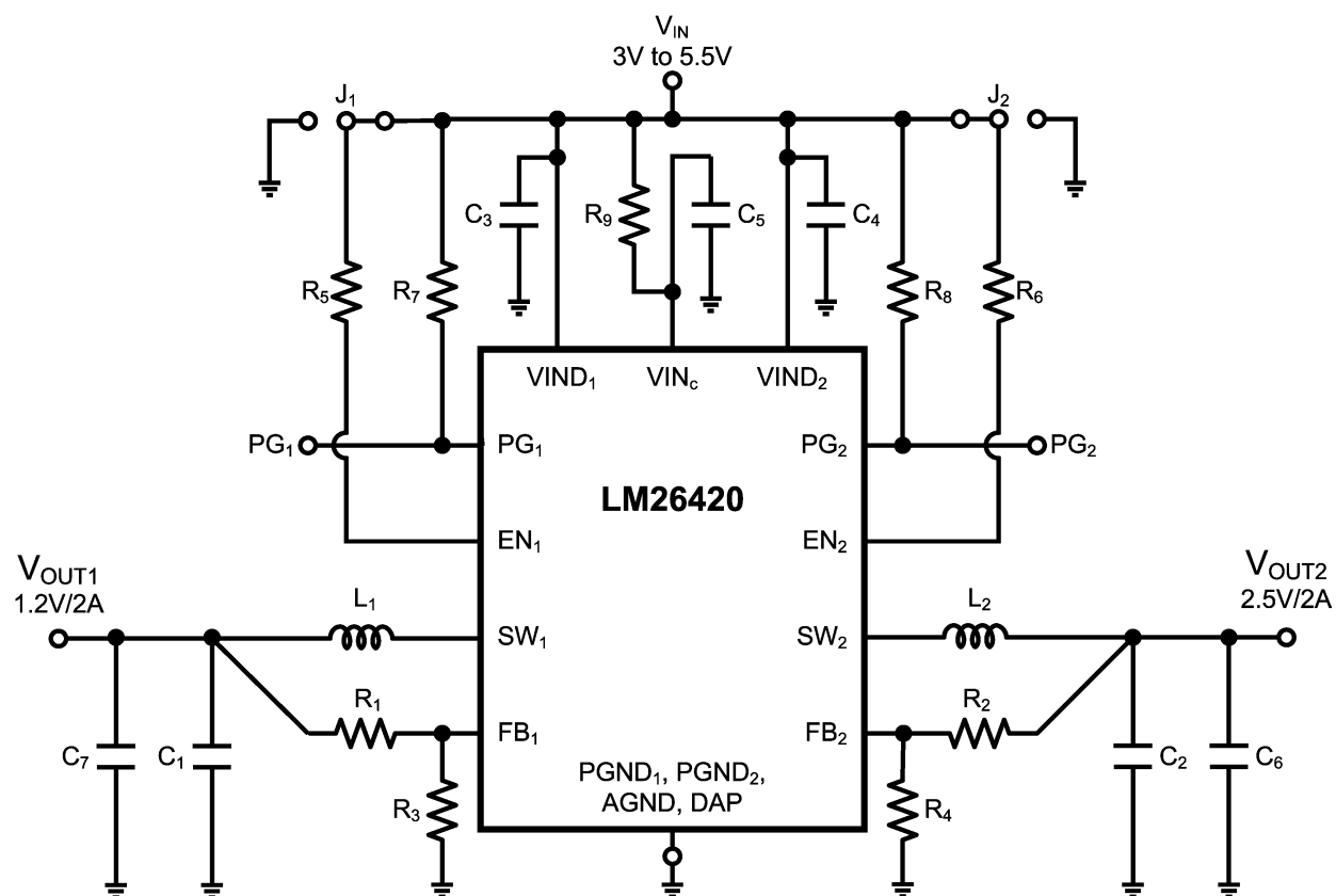
Figure 1. LM26420 Demo Board Schematic
