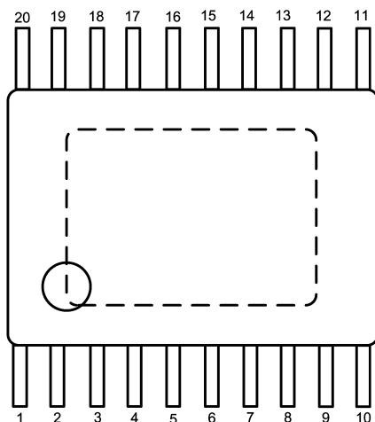
Figure 3. 20-Pin HTSSOP (top view)
