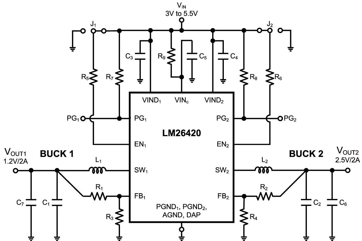
Figure 4. Schematic - X Version
