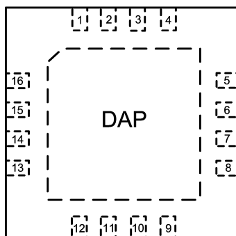
Figure 2. 16-Pin WQFN (top view)
