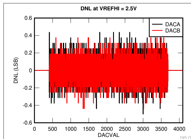
Figure 7-51. DNL
