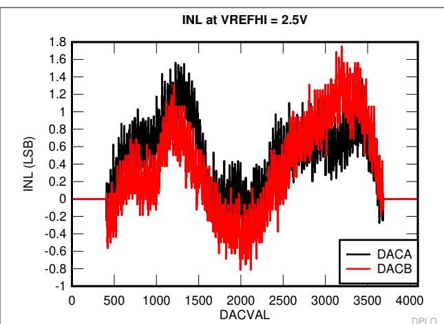
Figure 7-52. INL
