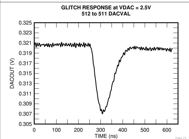
Figure 7-54. Glitch Response – 512 to 511 DACVAL
