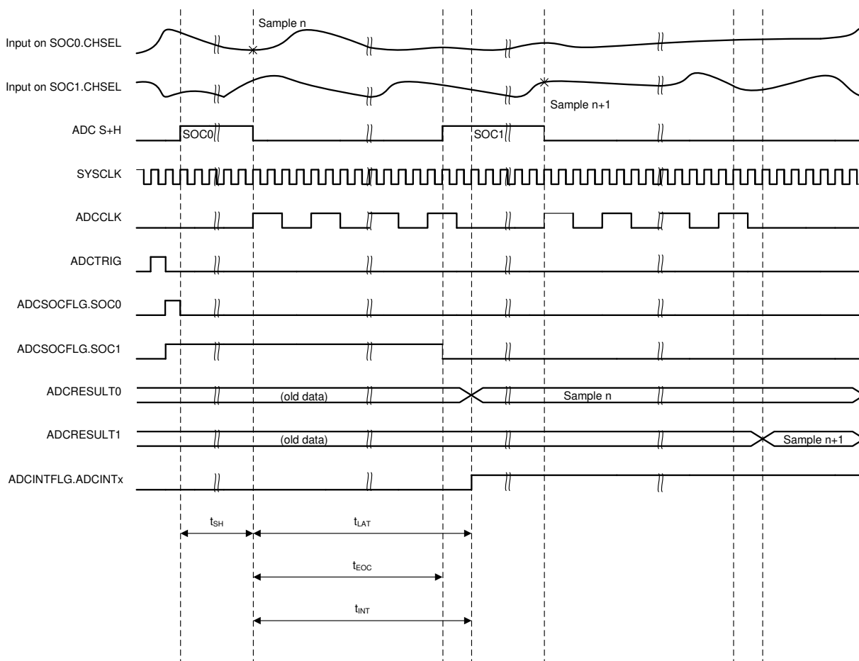
Figure 7-44. ADC Timings
