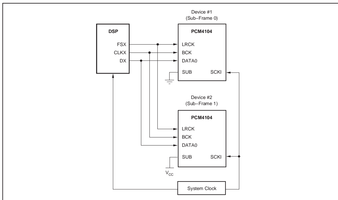
Figure 12. TDM Connection
