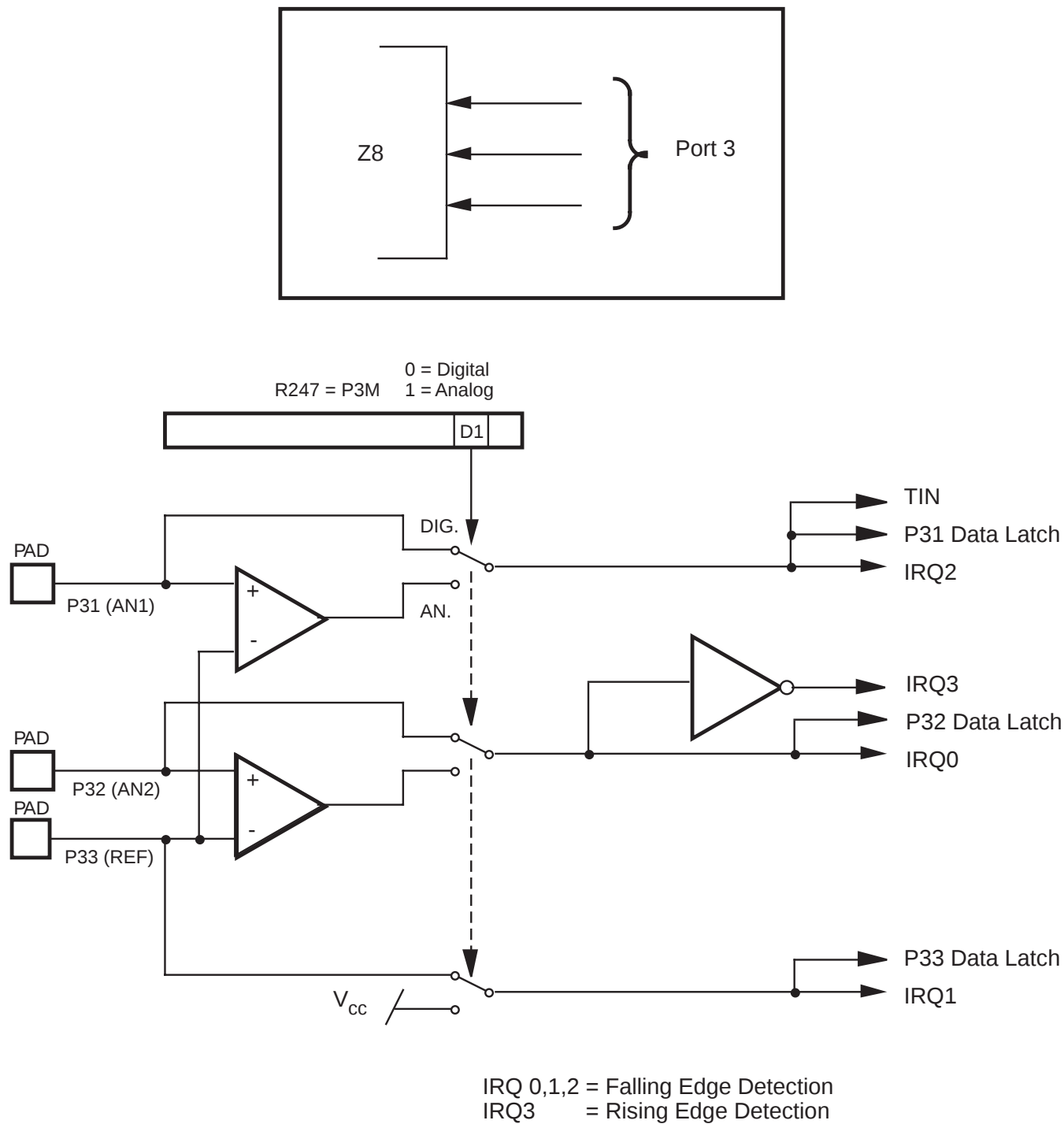
Figure 9. Port 3 Configuration
