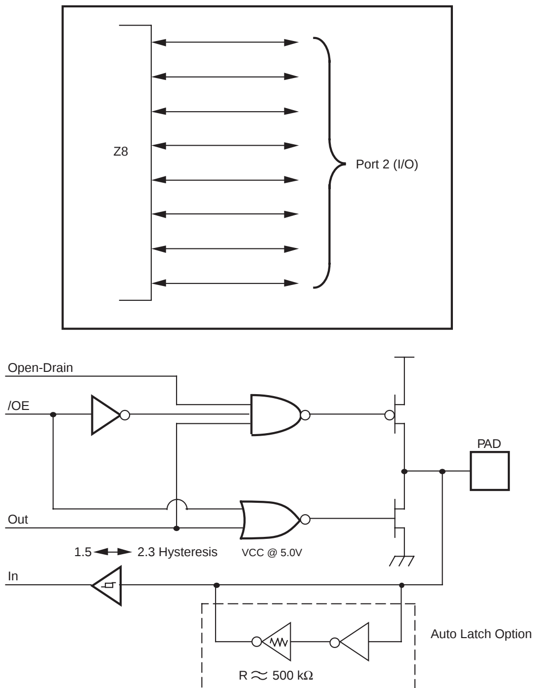
Figure 8. Port 2 Configuration
