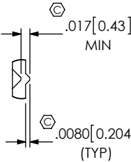
CRIMP DETAIL SCALE: 4:1 (TYP ALL CRIMPS)
