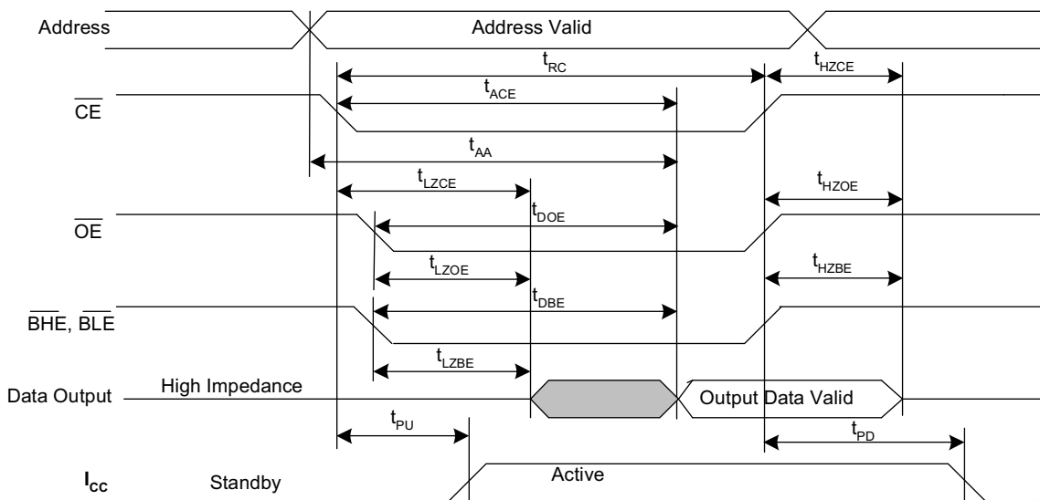
Figure 9. SRAM Read Cycle No. 2 ( \overline{\text{CE}} and \overline{\text{OE}} Controlled) [32, 34, 35]
