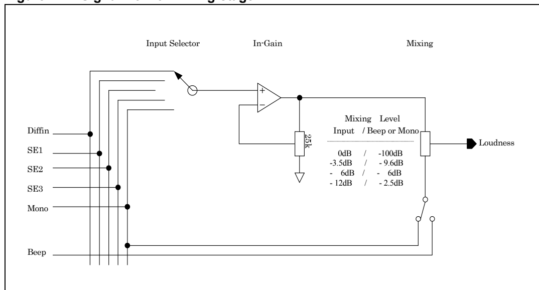
Figure 4. Signal-flow of mixing-stage
