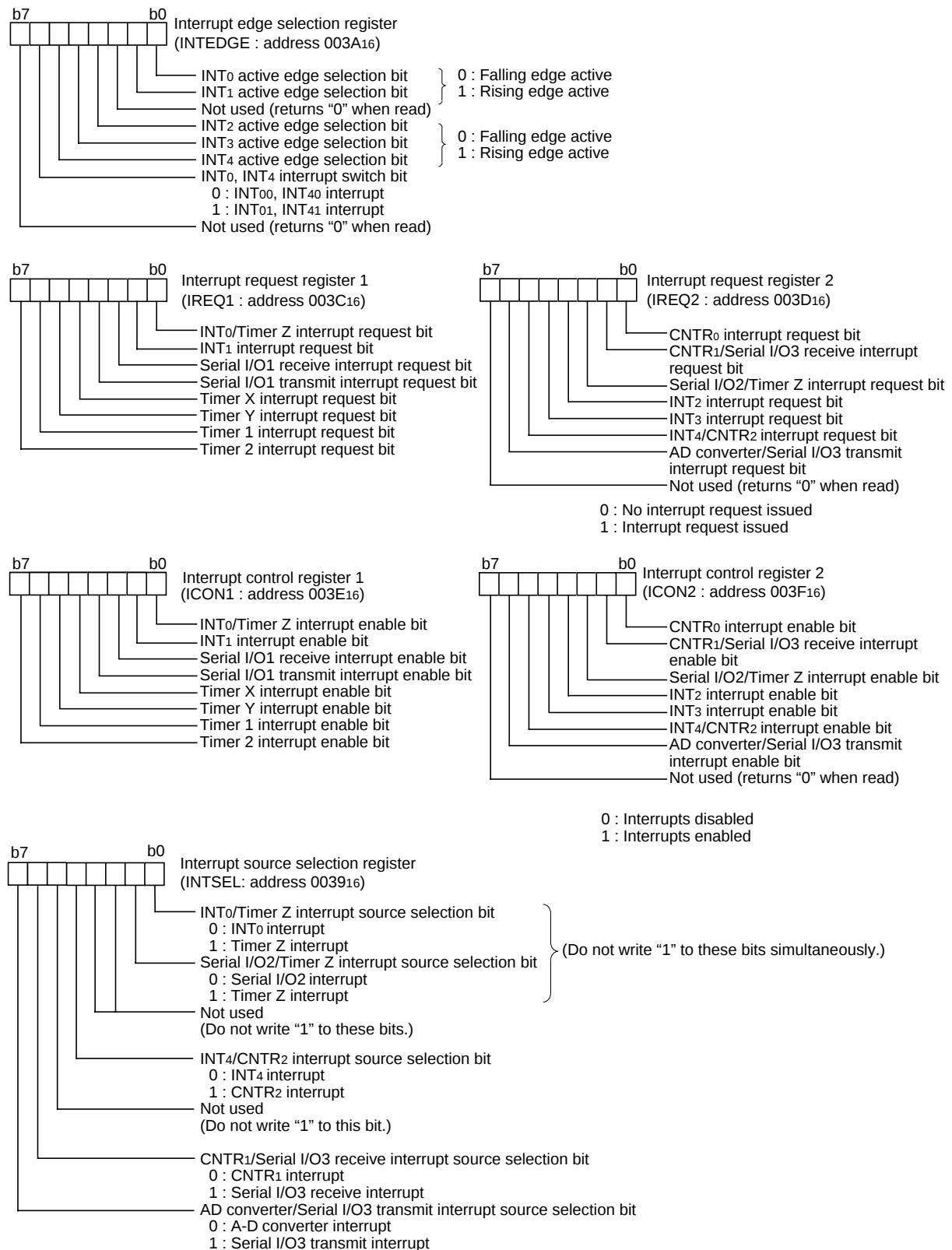
Fig. 27 Structure of interrupt-related registers of 3803 group
