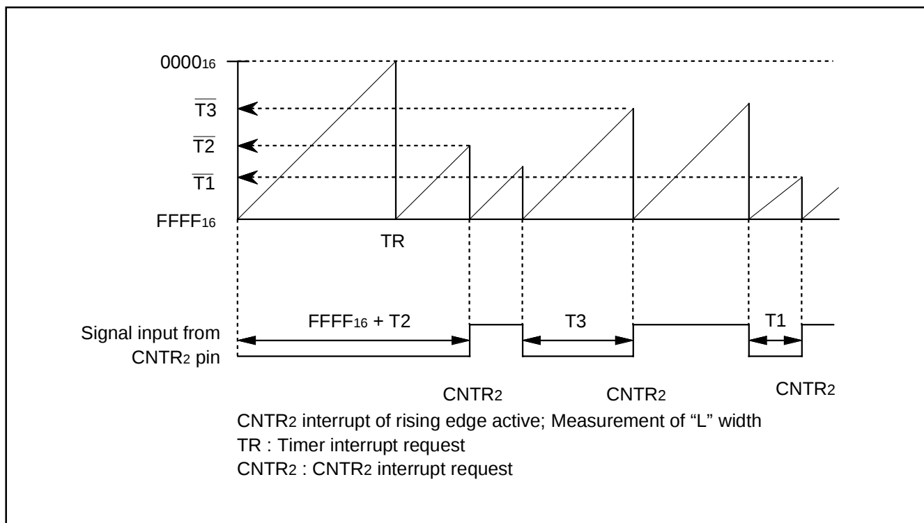
Fig. 37 Timing chart of pulse width measurement mode (Measuring "L" term)
