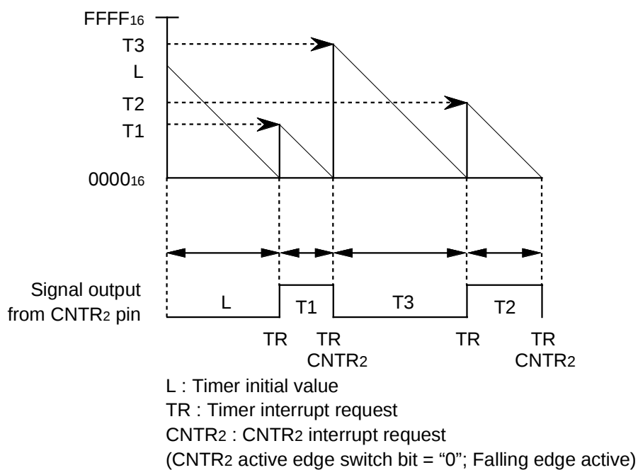
Fig. 38 Timing chart of programmable waveform generating mode
