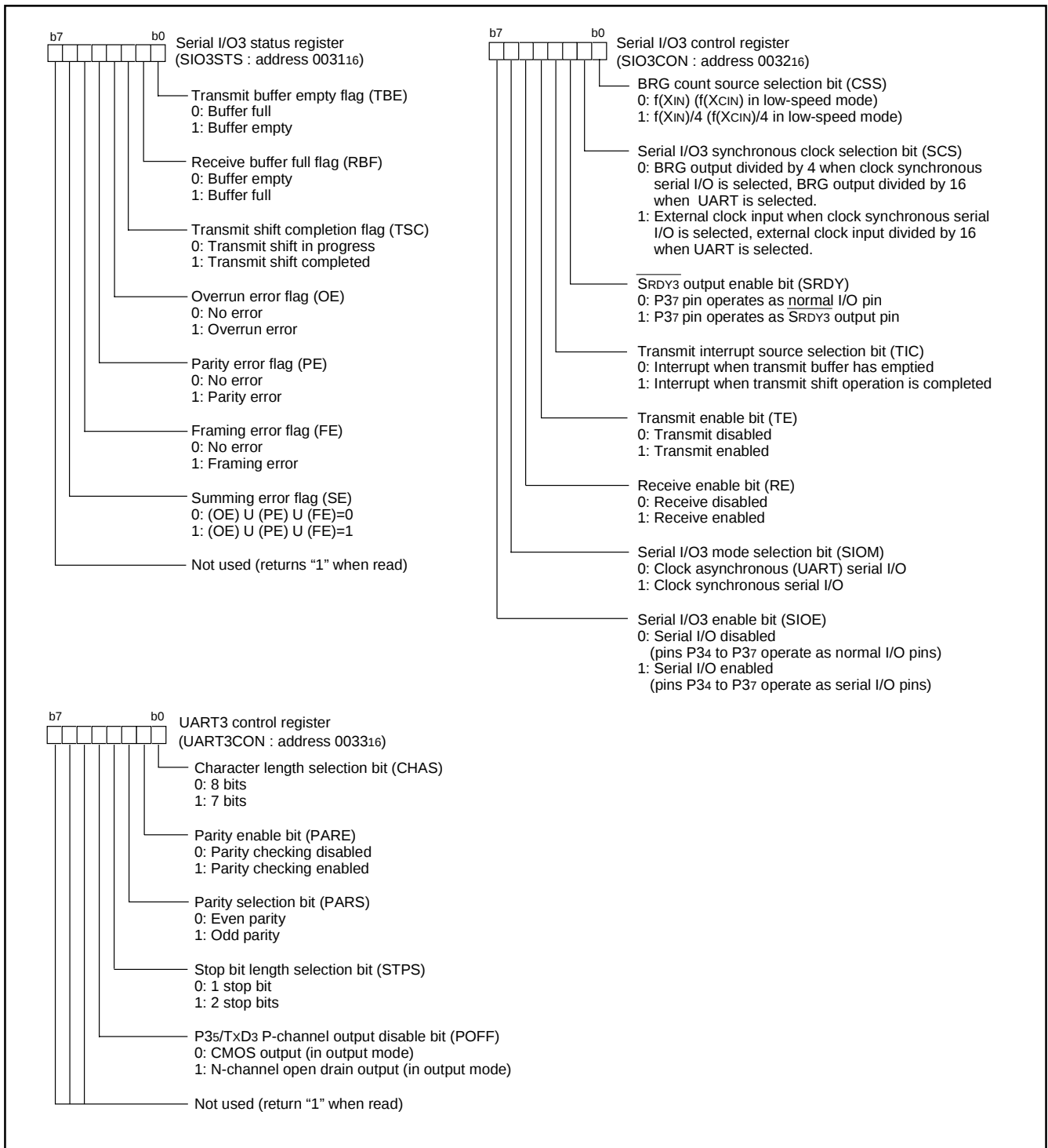
Fig. 52 Structure of serial I/O control registers
