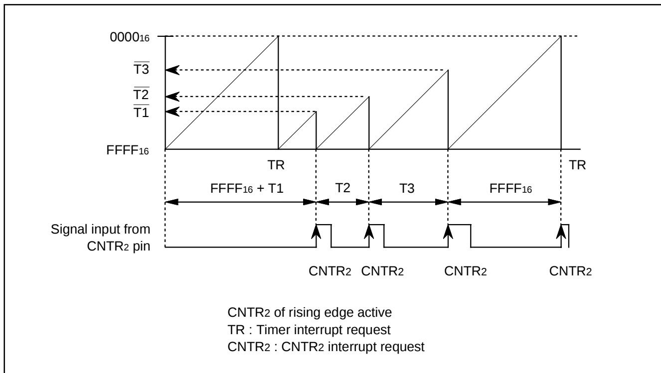
Fig. 36 Timing chart of pulse period measurement mode (Measuring term between two rising edges)
