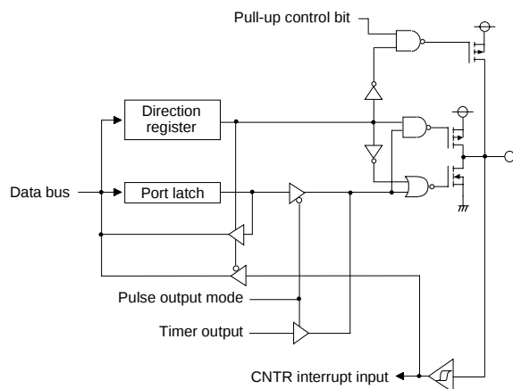
Fig. 21 Port block diagram of 3804 group (3)
