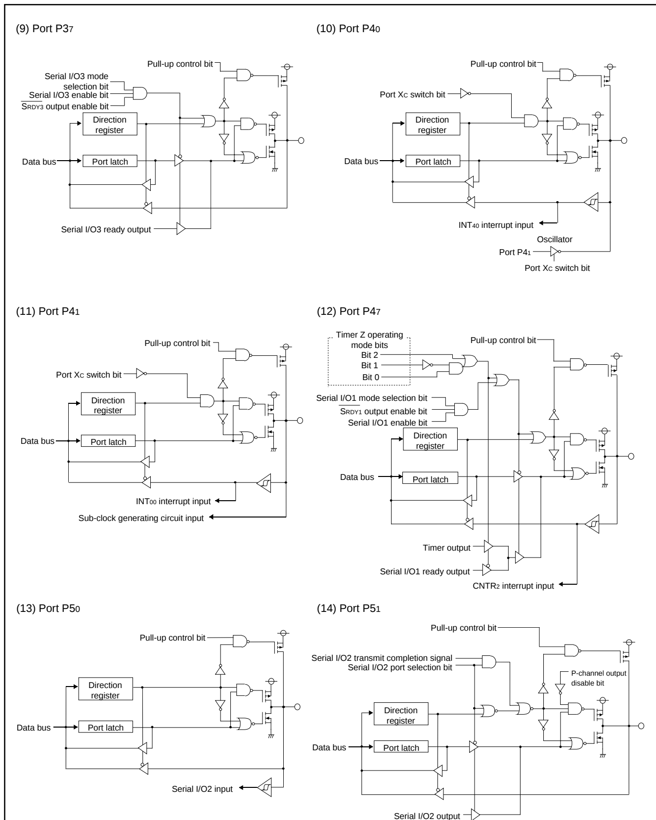
Fig. 20 Port block diagram of 3804 group (2)
