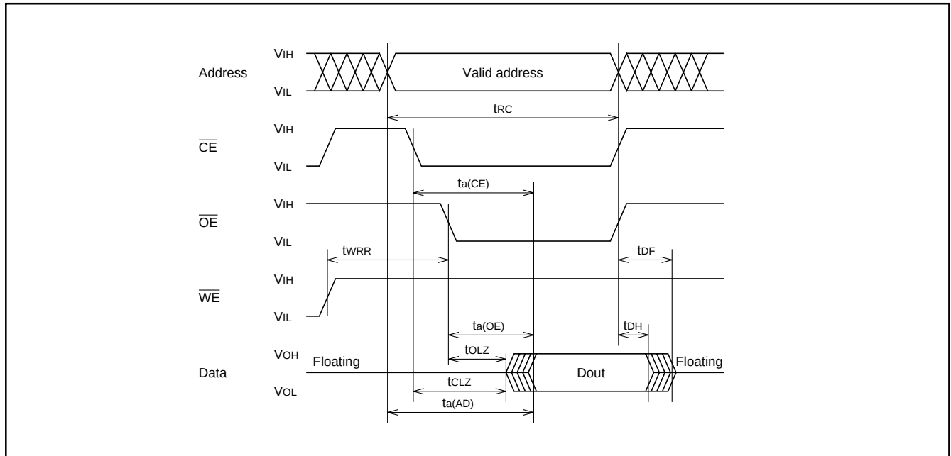
Fig. 88 Read timing
