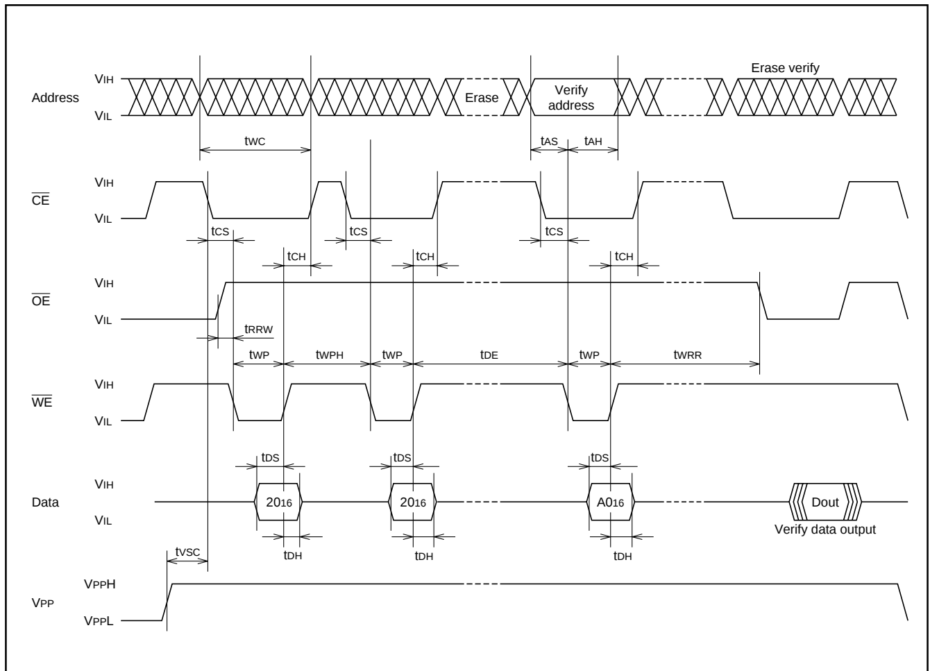
Fig. 91 Input/output timings during erasing (Verify data is output at the same timing as for read.)
