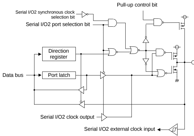
(17) Ports P54, P55
