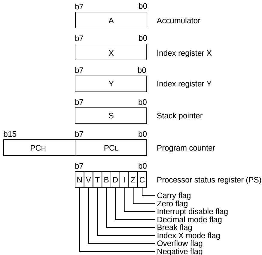
Fig.9 740 Family CPU register structure
