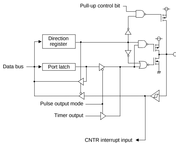
Fig. 18 Port block diagram of 3803 group (3)
