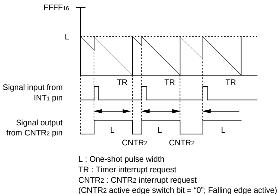
Fig. 39 Timing chart of programmable one-shot generating mode ("H" one-shot pulse generating)
