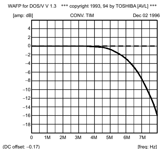
Figure 3 Y-signal 6M-LPF characteristics
