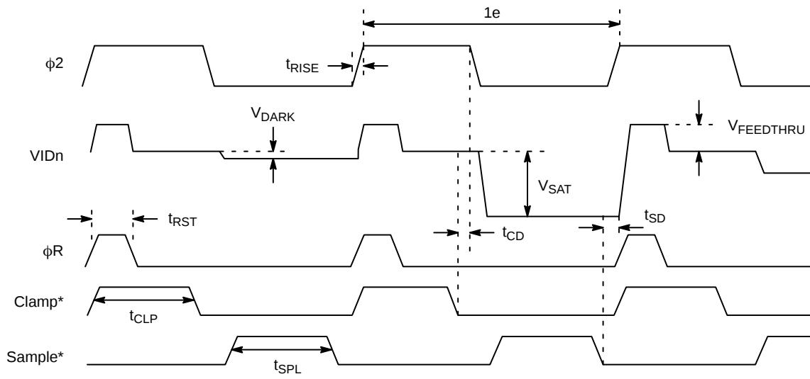
Figure 18. Output Timing
