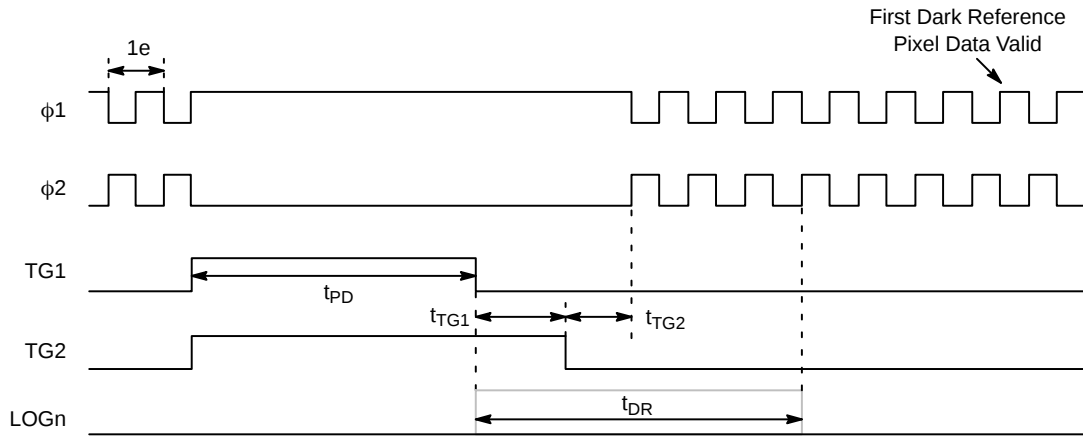
Figure 17. Photodiode-to-CCD Transfer
