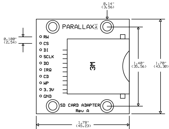
Figure 2: Module Dimensions
