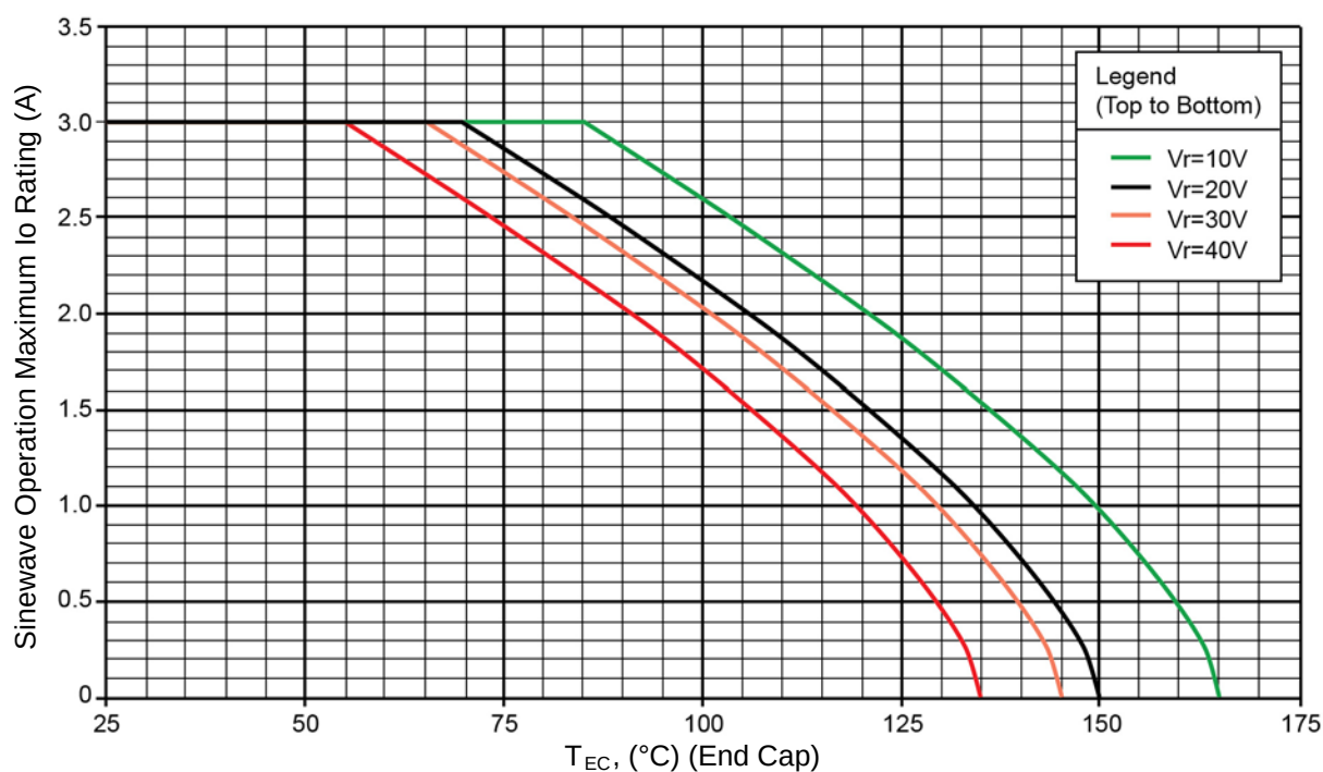
FIGURE 3 Temperature Current Derating For 1N5822US
