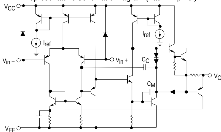
Representative Schematic Diagram (Each Amplifier)
