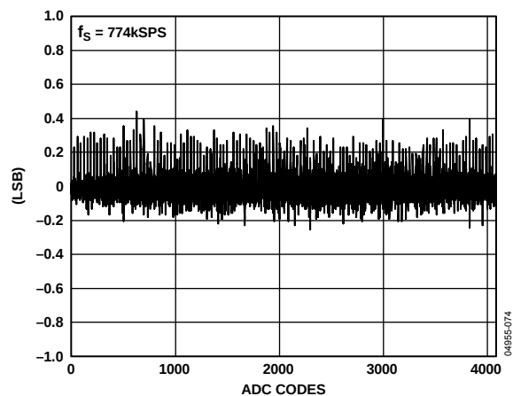
Figure 19. Typical DNL Error, f_s = 774 kSPS
