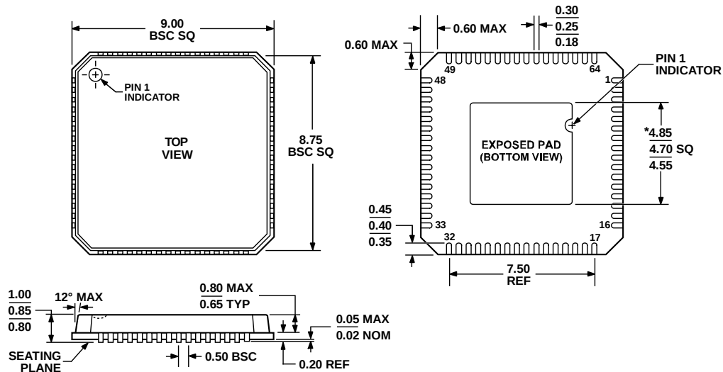
Figure 82. 64-Lead Frame Chip Scale Package [LFCSP_VQ]
