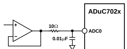
Figure 47. Buffering Single-Ended/Pseudo Differential Input
