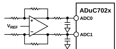
Figure 48. Buffering Differential Inputs
