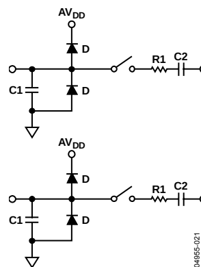
Figure 46. Equivalent Analog Input Circuit Conversion Phase: Switches Open; Track Phase: Switches Closed
