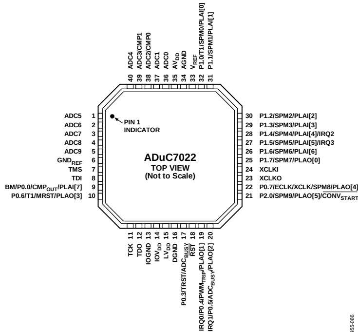
Figure 12. ADuC7022 40-Lead LFCSP_VQ Pin Configuration
