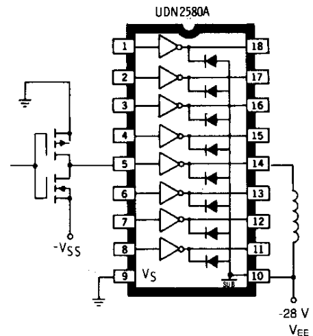
TELECOMMUNICATIONS RELAY DRIVER (Negative Logic)
