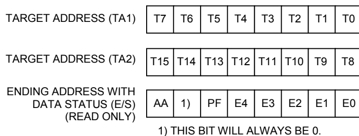
Figure 6. ADDRESS REGISTER
