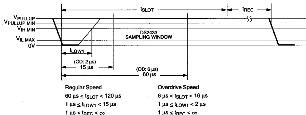
Figure 11. READ/WRITE TIMING DIAGRAM Write-one Time Slot
