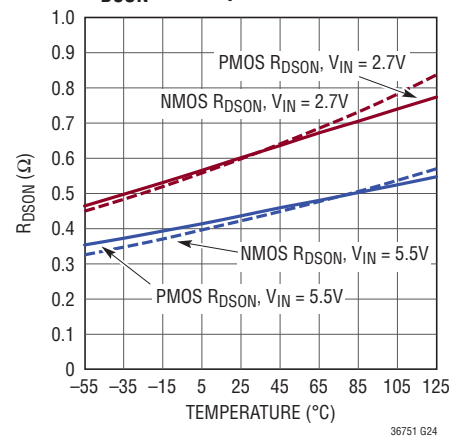
500mA Buck Regulators, Switch R_{DS(on)} vs Temperature
