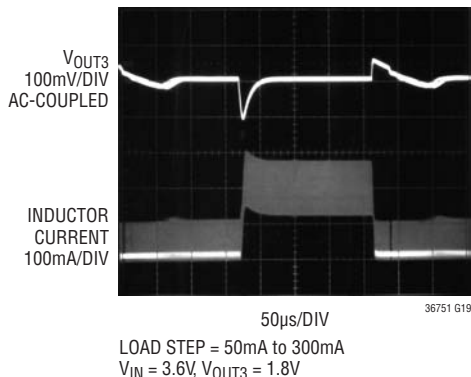
500mA Buck Regulators Transient Response (Pulse-Skipping Mode)
