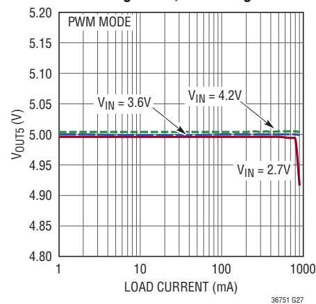
Boost Regulator, Load Regulation
