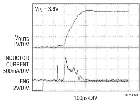
Buck-Boost Regulator No Load Start-Up (PWM Mode)
