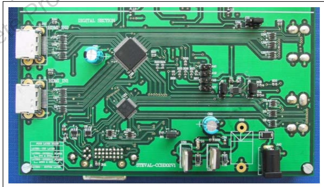
Figure 2. Digital section
