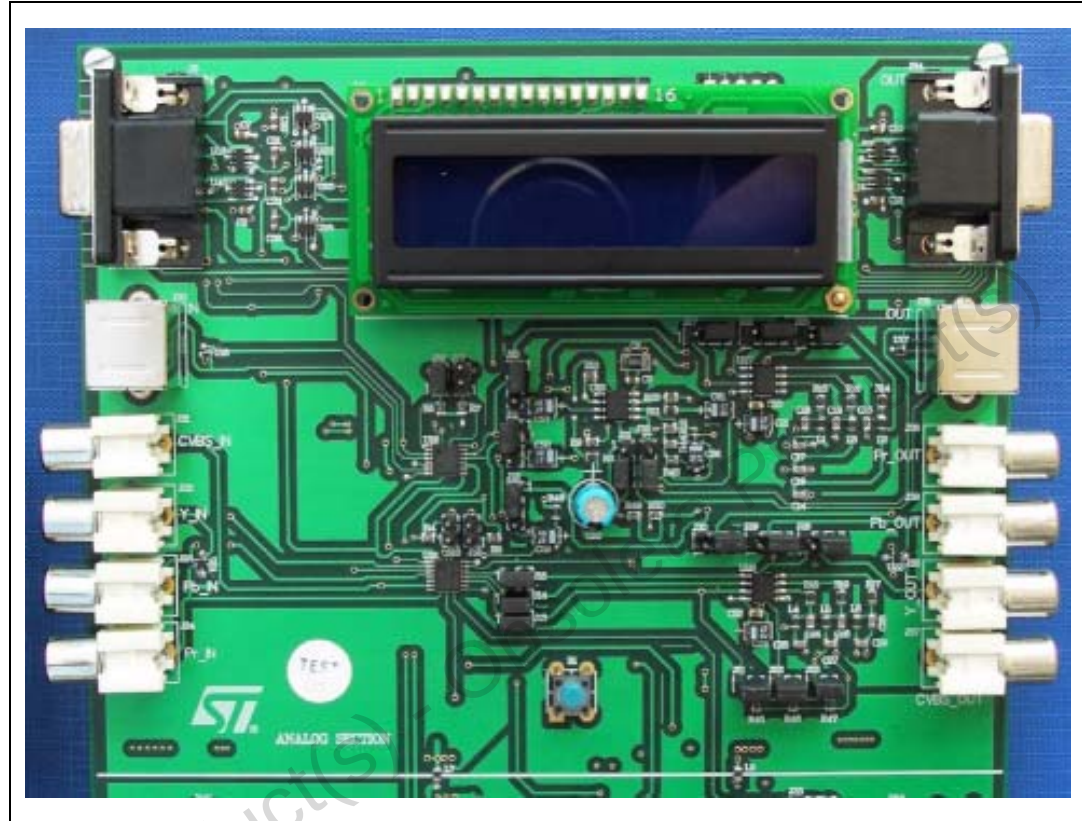
Figure 1. Analog section
