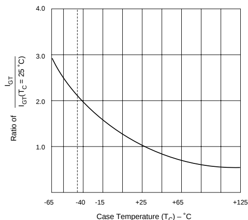
Figure E2.11 Normalized DC Gate Trigger Current for All Quadrants versus Case Temperature
