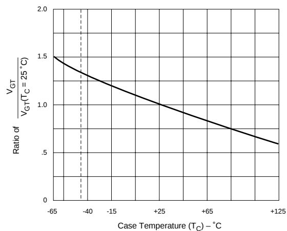
Figure E2.12 Normalized DC Gate Trigger Voltage for All Quadrants versus Case Temperature
