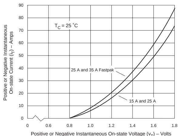
Figure E2.10 On-state Current versus On-state Voltage (Typical) (15 A and 25 A)
