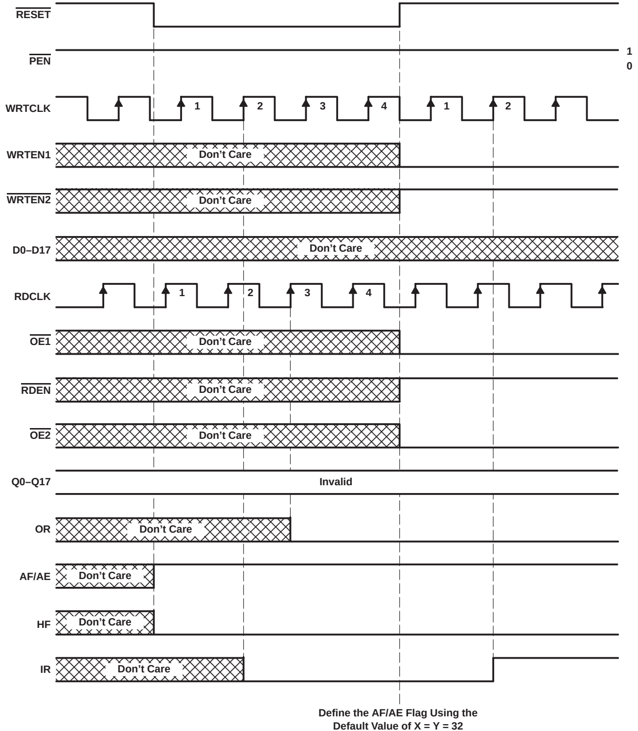
Figure 1. Reset Cycle
