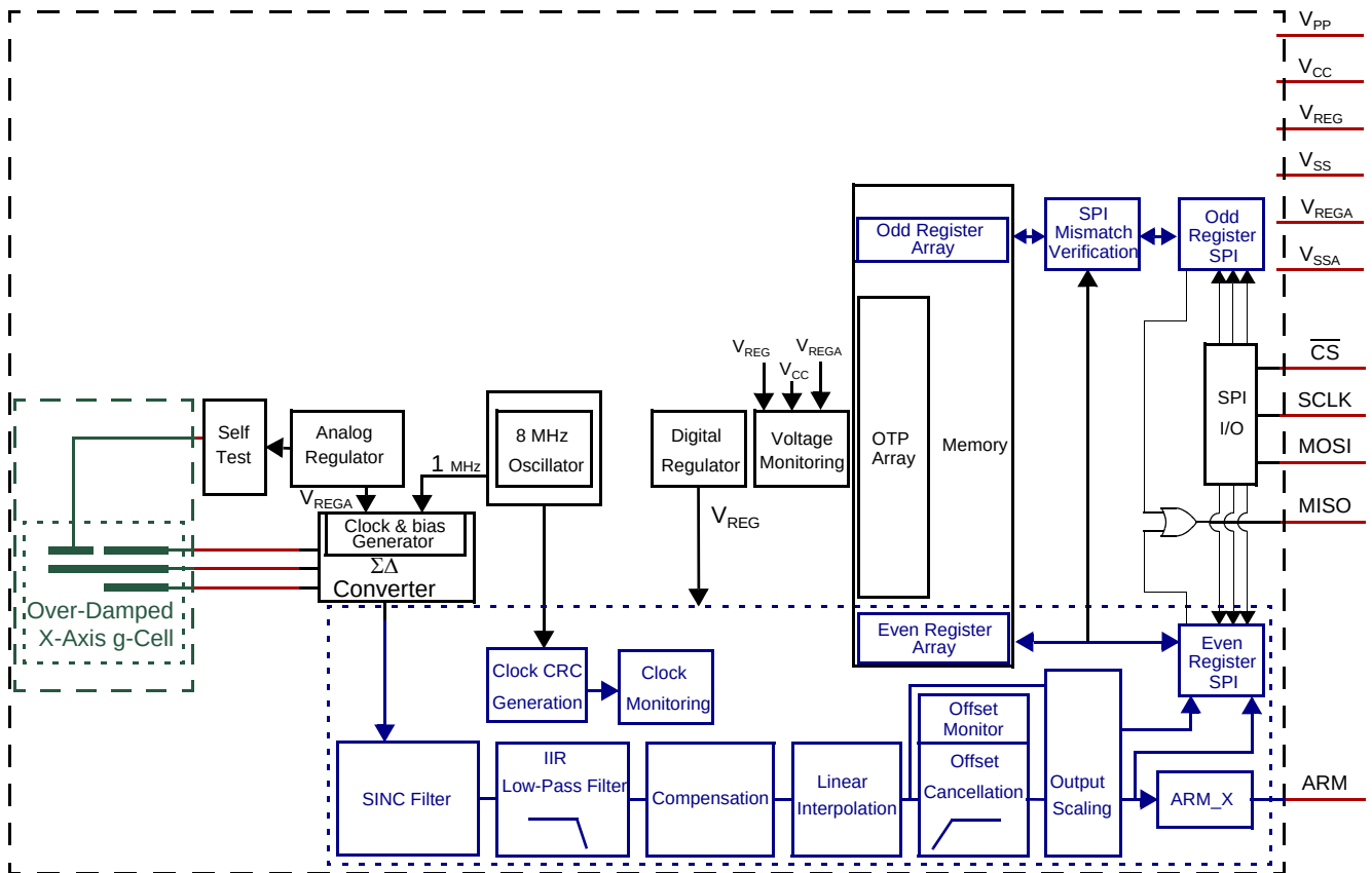
Figure 3. Block Diagram
