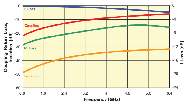
CP0402PxxxxBNTR
