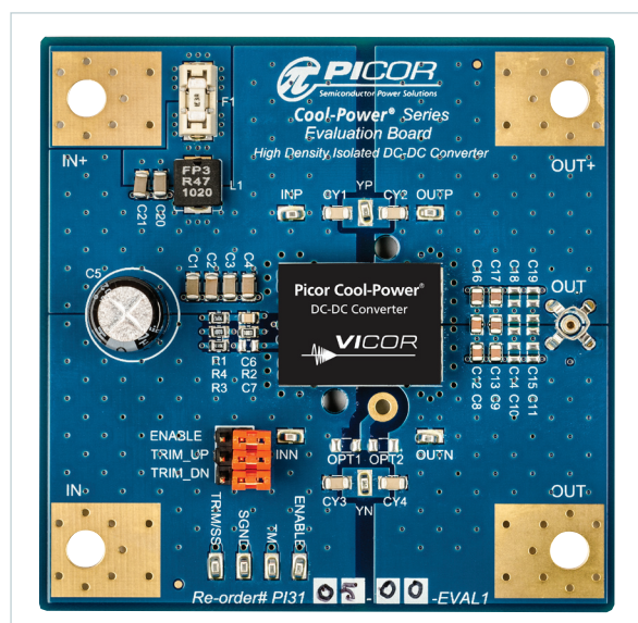
Figure 1. PI31xx-xx-EVAL1 Evaluation Board
