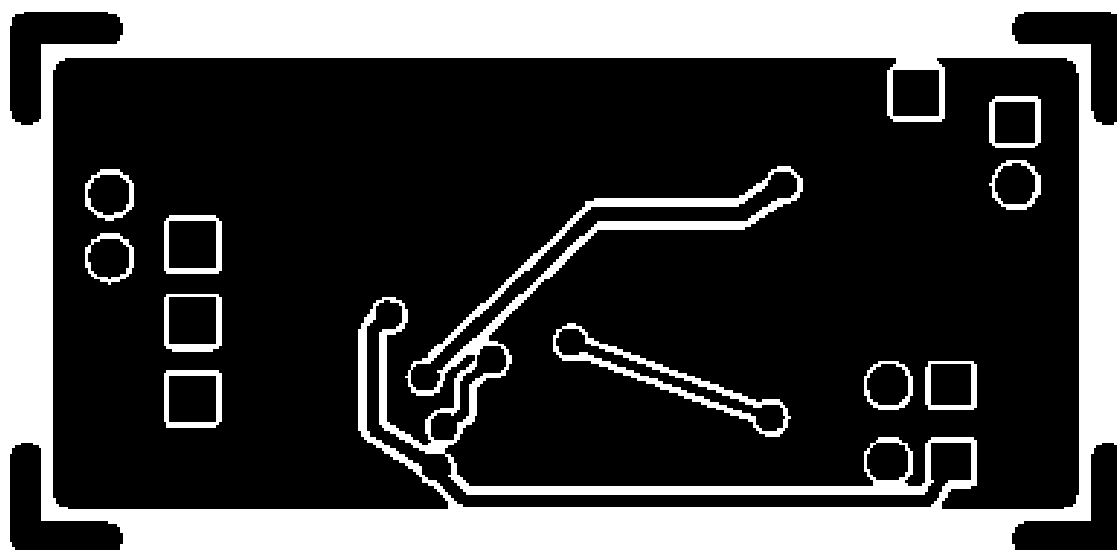
Figure 9. Bottom Layer
