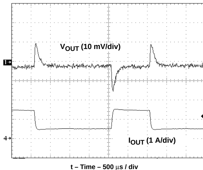
Figure 6. Transient Response
