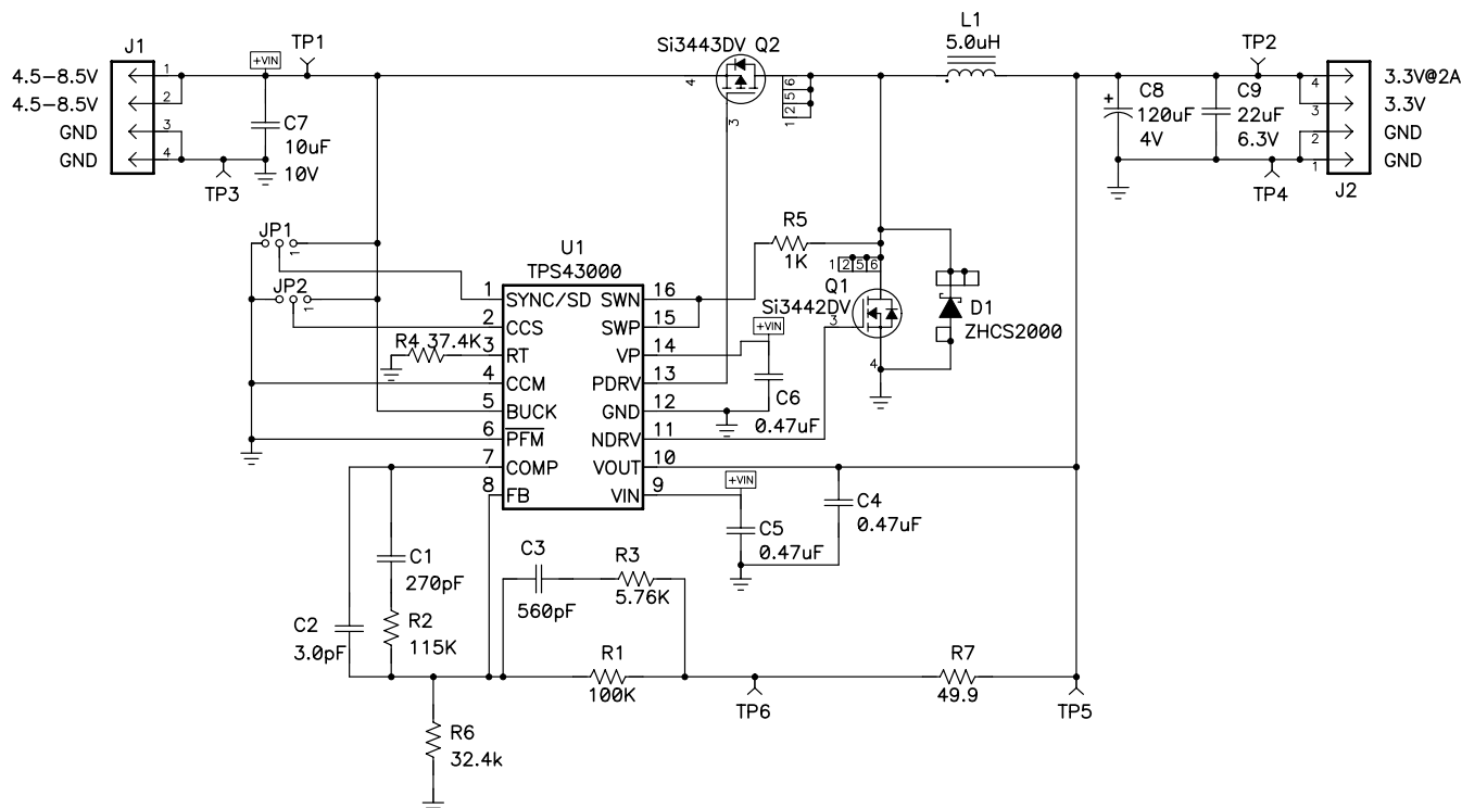
Figure 1. TPS43000-001EVM Schematic
