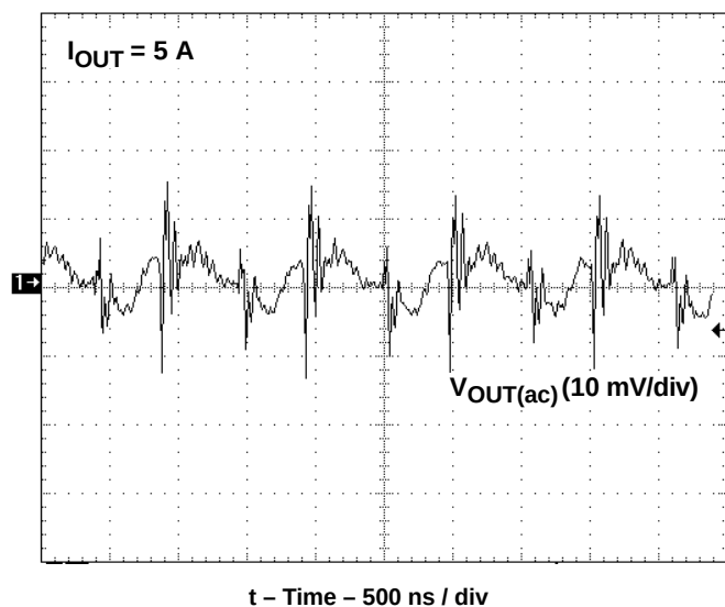
Figure 5. Output Ripple
