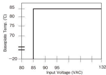
PF500A-360 (At 100% Load)
