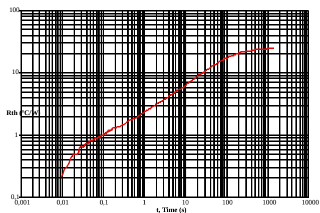
Figure 22. 33886 Thermal Response
