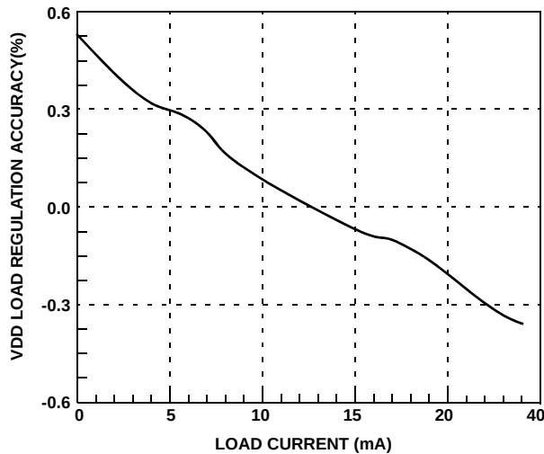
FIGURE 1. VDD LOAD REGULATION
