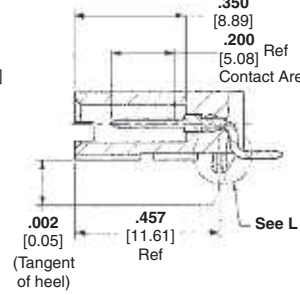
Section K-K
