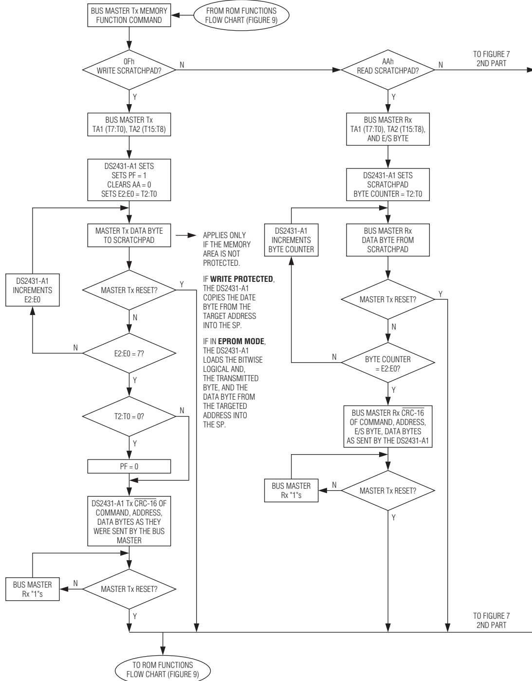
Figure 7. Memory Function Flow Chart
