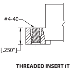
THREADED INSERT (T)
