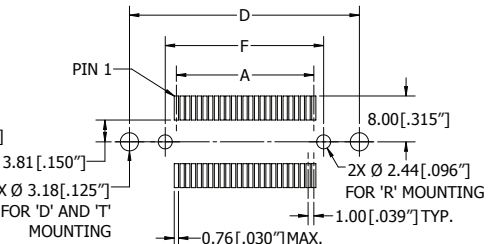
SURFACE MOUNT (HF)
