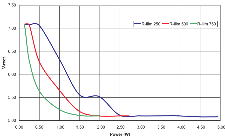
Figure 9. bq51013AEVM-765 V-rect vs Output Power
