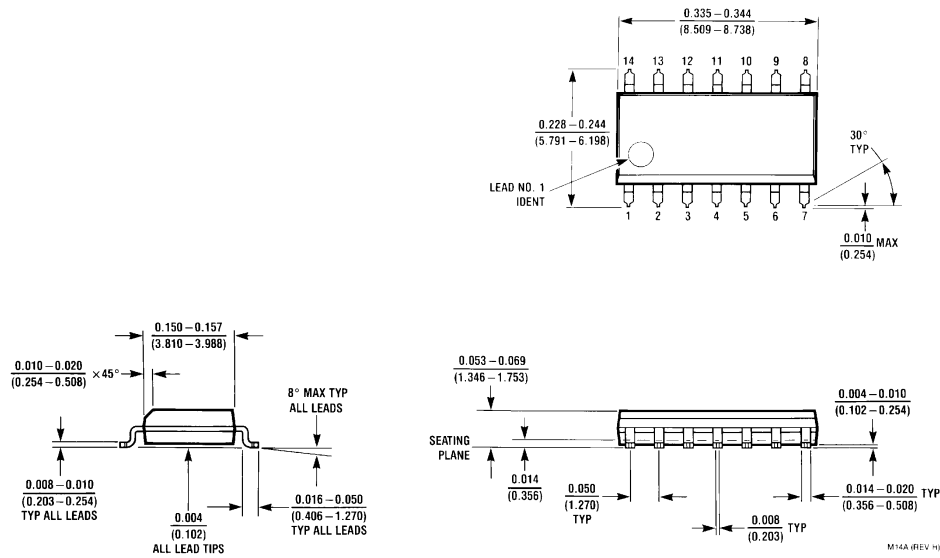
14-Lead Small Outline Package JEDEC (M) Order Number 74LCX00M or 74LCX00MX NS Package Number M14A
