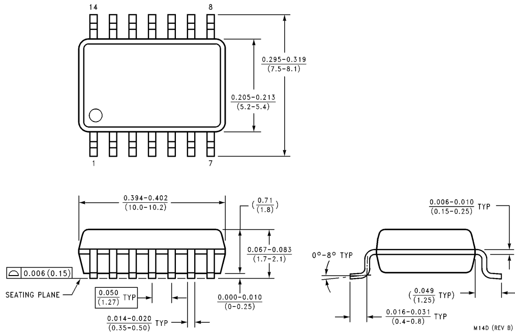
14-Lead Small Outline Package EIAJ (SJ) Order Number 74LCX00SJ or 74LCX00SJX NS Package Number M14D
