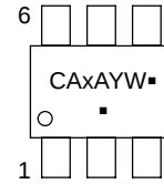
SOT-23-6 (TSOP-6) SN SUFFIX CASE 318G
