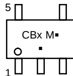
SC70-5 SQ SUFFIX CASE 419A
