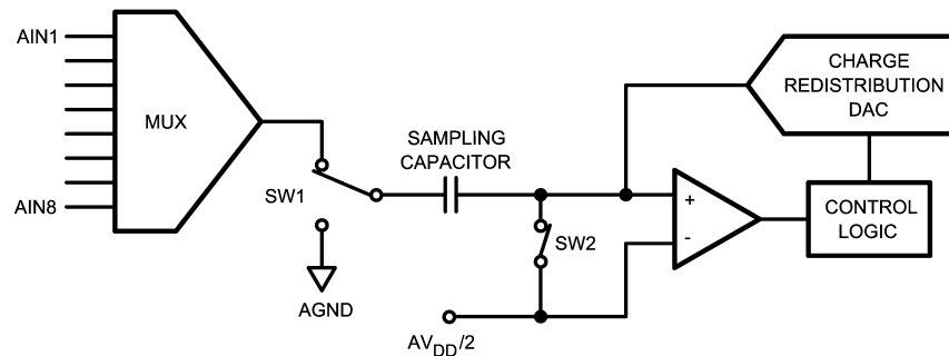
FIGURE 2. ADC78H90 in Track Mode
