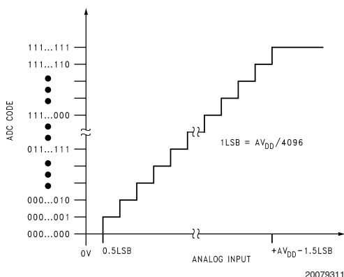
FIGURE 4. Ideal Transfer Characteristic
