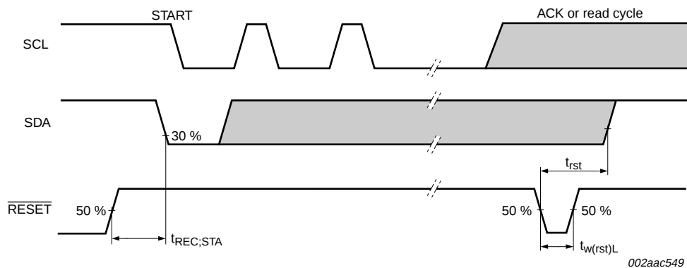
Fig 16. Definition of RESET timing
