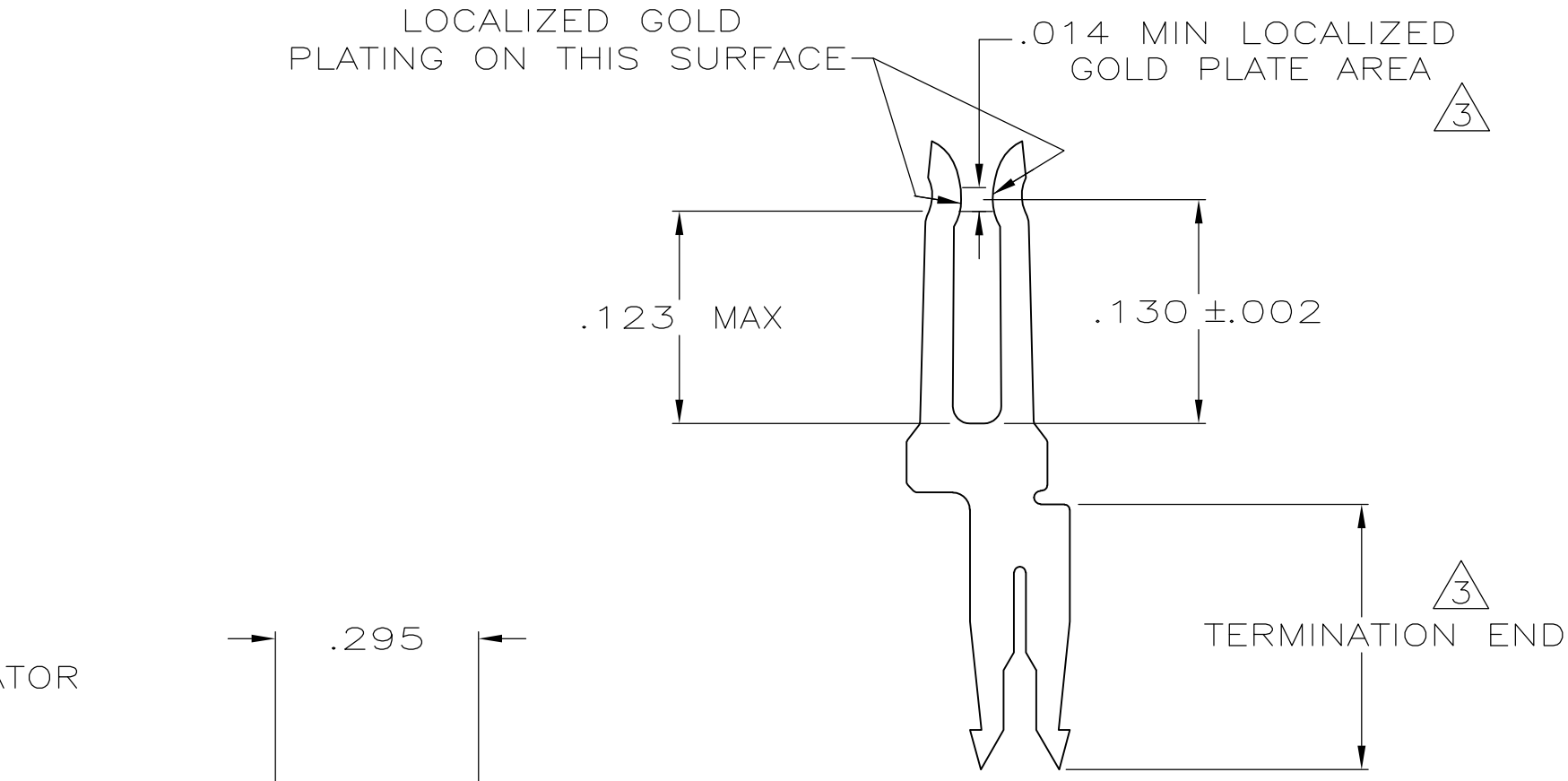
DETAIL Z SCALE 10:1 TYPICAL
