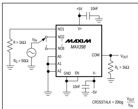
Figure 7. Crosstalk
