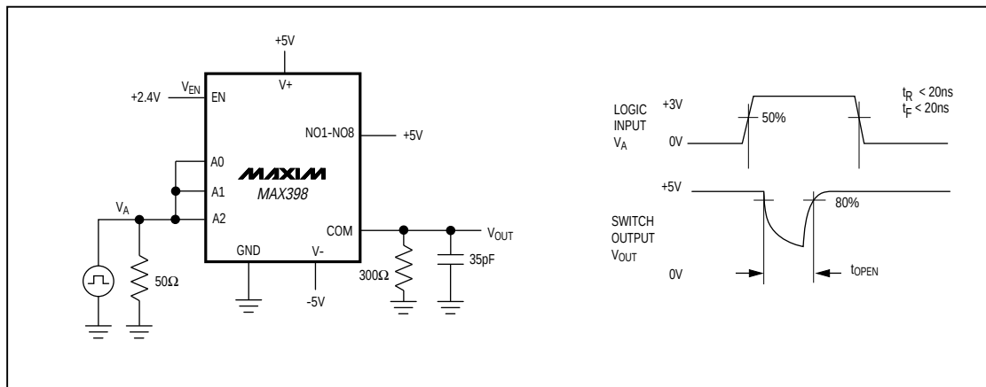
Figure 4. Break-Before-Make Interval
