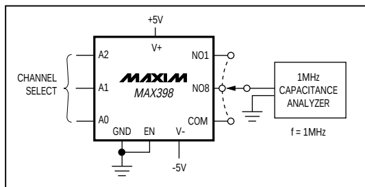
Figure 8. NO/COM Capacitance
